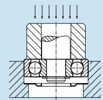
Correct method of fitting deep groove ball bearings.
