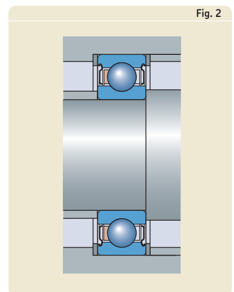
Recommended means of support for shields of 2Z/VA228 och 2Z/VA208 bearings
